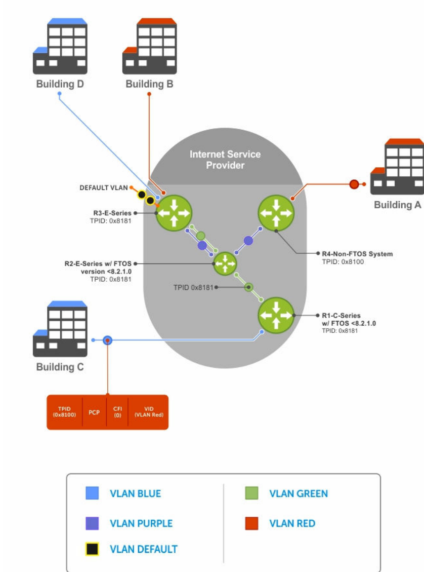
Figure 106. Single and Double-Tag First-byte TPID Match
